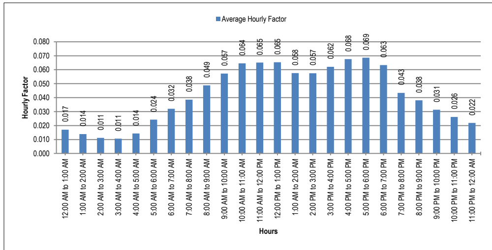
Figure 3-8: Hourly Factor on N-5
