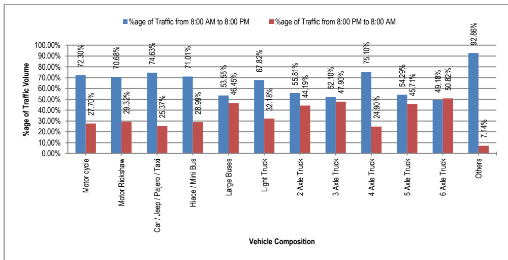
Figure 5-9: Percentage of Traffic Composition in Day and Night Time on N-45
