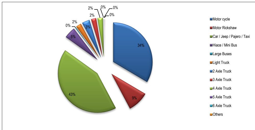
Figure 5-4: Percentage of Vehicle Composition in NB Direction of N-45
