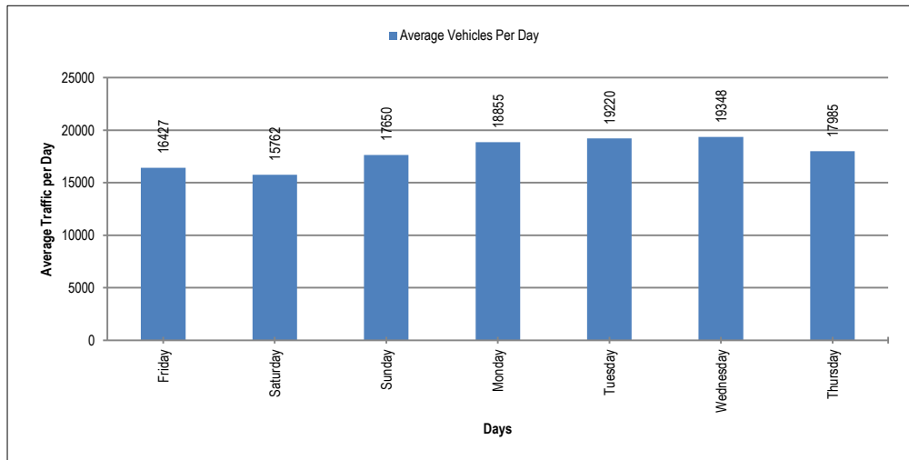
Figure 3-7: Weekly Trend of Traffic on N-5
