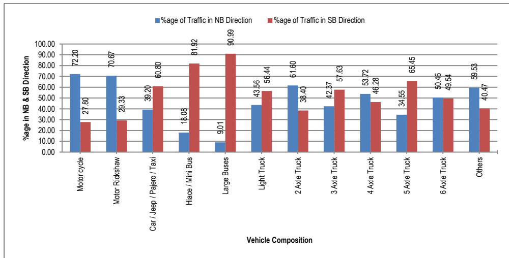
Figure 5-6: Directional Distribution of Traffic Volume on N-45
