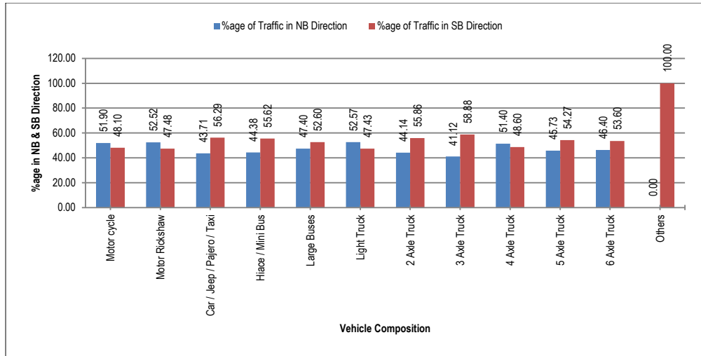
Figure 4-6: Directional Distribution of Traffic Volume on N-35
