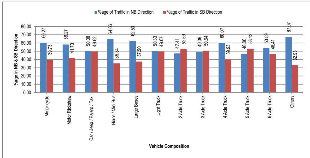
Figure 3-6: Directional Distribution of Traffic Volume on N-5
