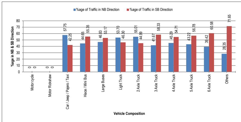
Figure 2-6: Directional Distribution of Traffic Volume on M-1
