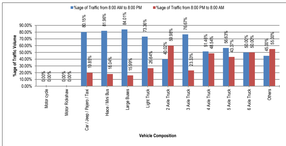
Figure 2-9: Percentage of Traffic Composition in Day and Night Time on M-1
