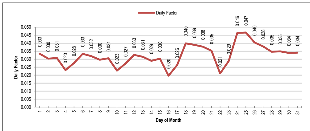
Figure 3-3: Daily Traffic Factor on N-5
