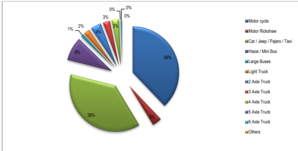
Figure 3-4: Percentage of Vehicle Composition in NB Direction of N-5
